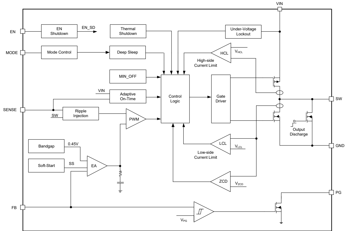
Figure 2. Block Diagram
