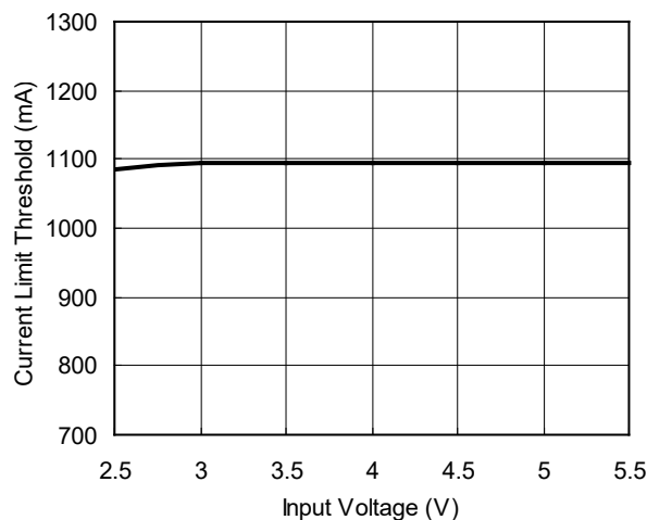
Current Limit Threshold vs. Input Voltage (SGM2581E/F/K)
