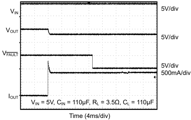
Resistance Load Inrush Response (SGM2581A/B/G)
