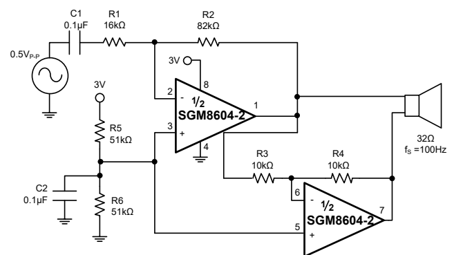
Figure 2. SGM8604-2 Bridge Amplifier for 200mW at 3V
