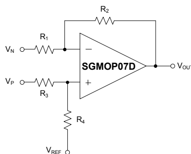
Figure 2. Differential Amplifier
