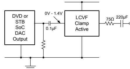
Figure 3. AC-Coupled Inputs and Outputs
