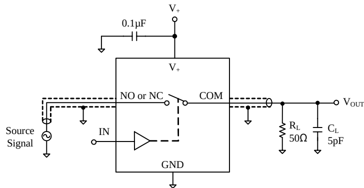
Test Circuit 7. Off Isolation
