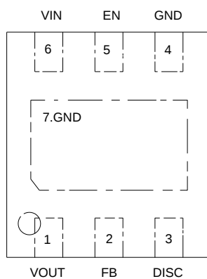
Figure 3kTDFN6-2x2(TD) package
