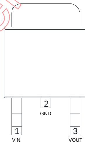
Figure 3oTO-252(O2) package
