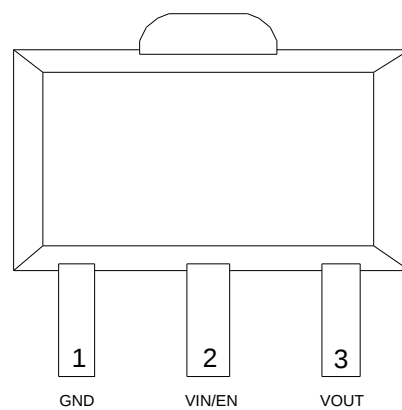
Figure 3i SOT-89-3(S9) package
