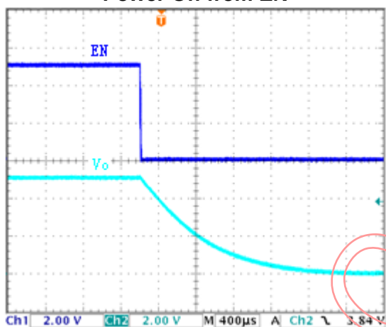
Power Off from EN
