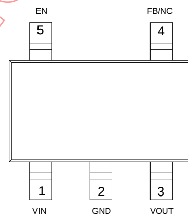
Figure 3f SOT-23-5(SX) package
