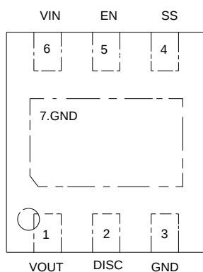
Figure 3mTDFN6-2x2(D2) package
