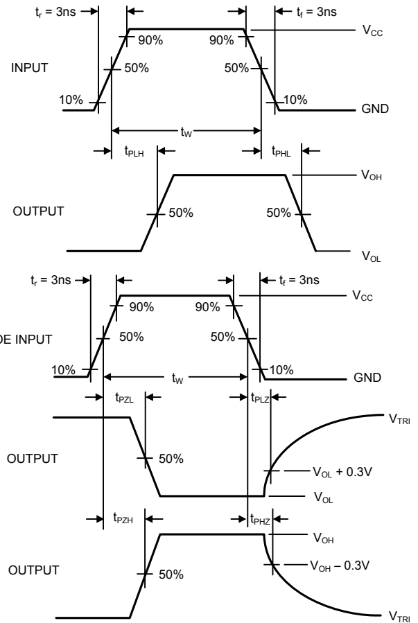
Figure 2. AC Waveforms
