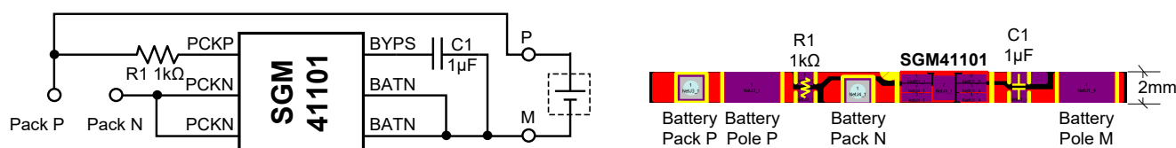
Figure 1. Typical Application Circuit and Demonstration Board Outline
