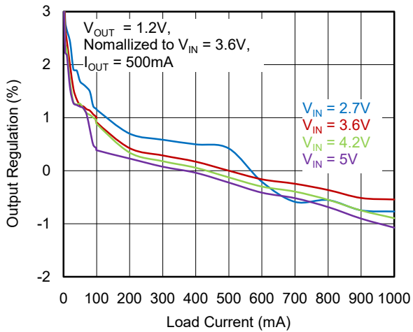
\Delta V_{OUT} (\%) vs. Load Current
