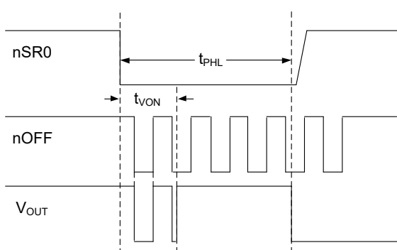
图 11. Timing Diagram ( nSR0 + nOFF vs. V_{OUT} )
