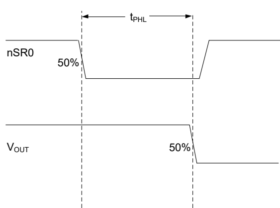
图 10. Turn-Off with nSR0 2
