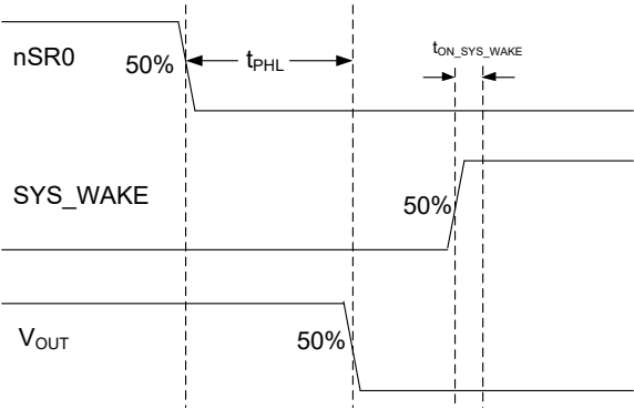
图 15. Timing Diagram (nSR0 + SYS_WAKE vs. V_OUT) 1
