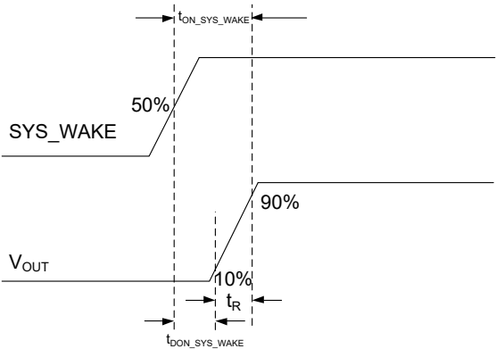
图 13. Timing Diagram (SYS_WAKE vs. V_OUT)
