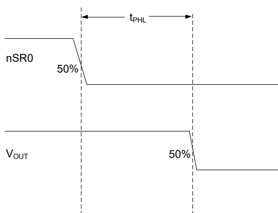
图 9. Turn-Off with nSR0 1
