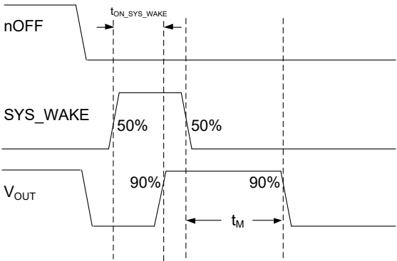
图 14. Timing Diagram (nOFF + SYS_WAKE vs. V_OUT)
