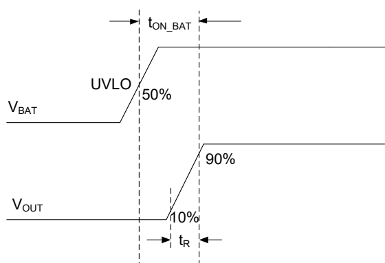
图 7. Timing Diagram ( V_{BAT} vs. V_{OUT} )
