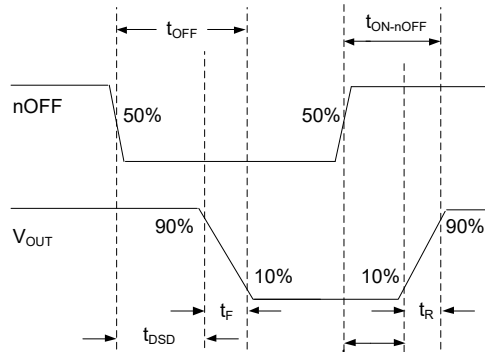
图 12. Timing Diagram ( nOFF vs. V_{OUT} )
