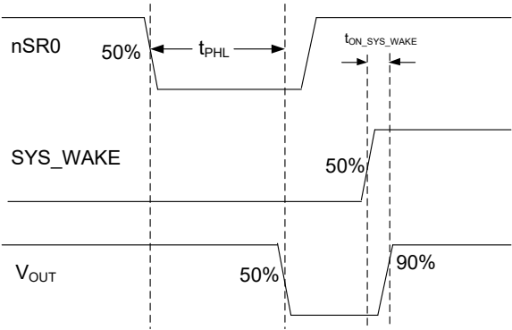
图 16. Timing Diagram (nSR0 + SYS_WAKE vs. V_OUT) 2
