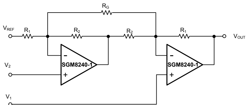
Figure 6. High-side Current Measurement
