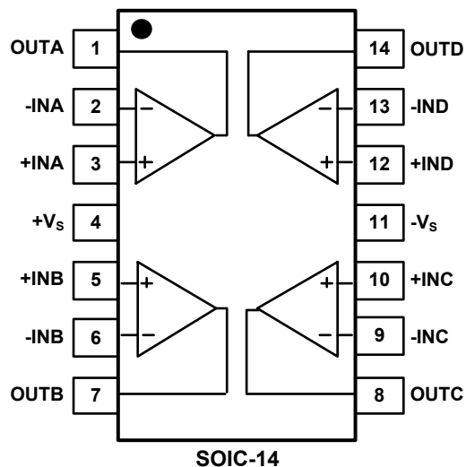
SGM8240-4 (TOP VIEW)
