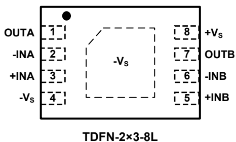
SGM8240-2 (TOP VIEW)
