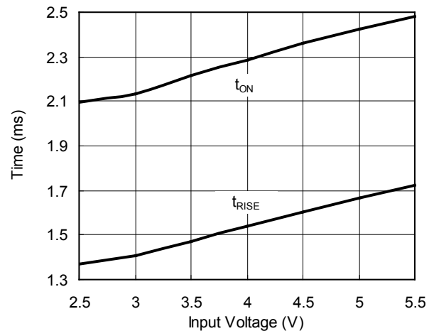
Turn-On (Rise) Time vs. Input Voltage
