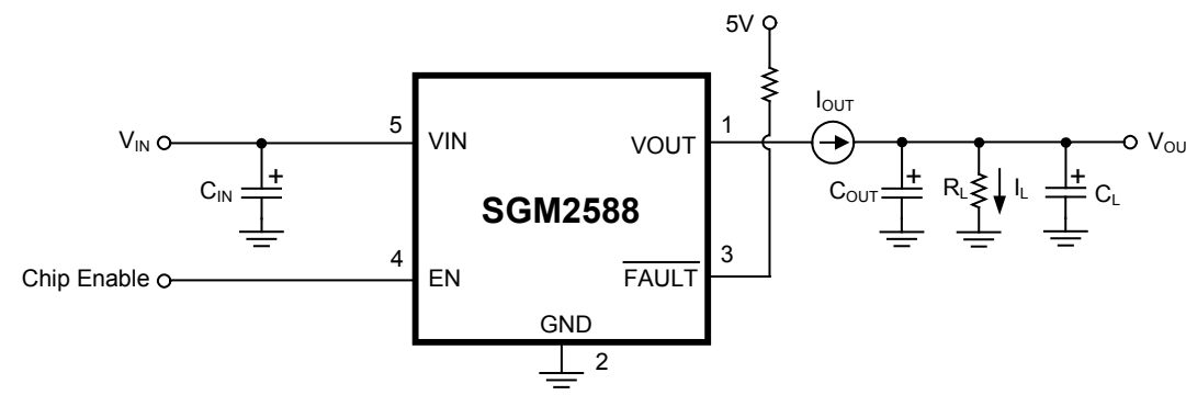
Figure 2. SGM2588 Test Circuit
