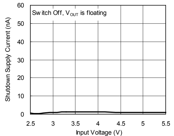
Shutdown Supply Current vs. Input Voltage
