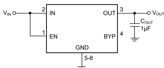
Figure 6. Low Noise Fixed Voltage Regulator
