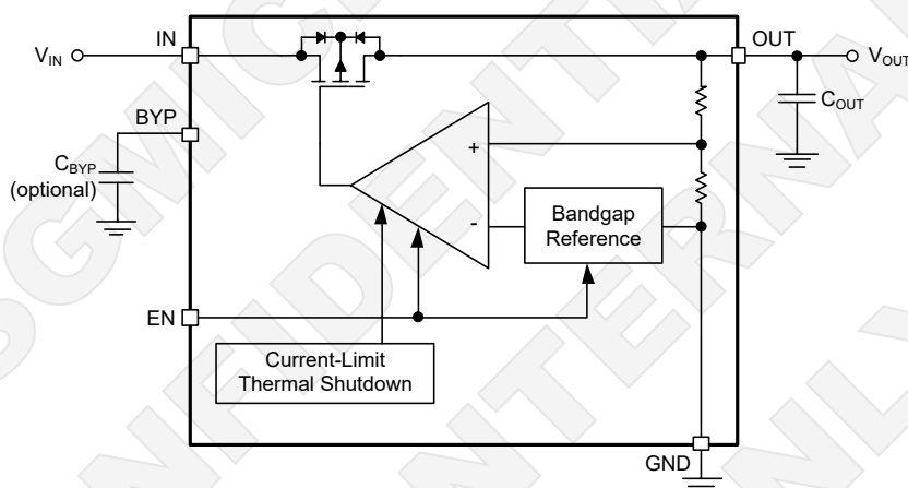
Figure 4. Ultra Low Noise Fixed Regulator (SOIC-8 and TO-263-5B Versions)
