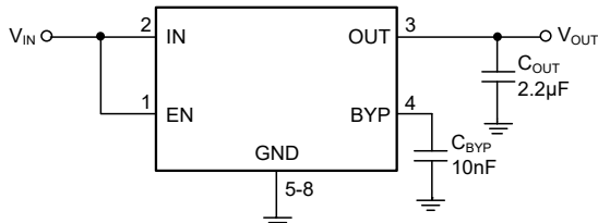
Figure 7. Ultra Low Noise Fixed Voltage Regulator
