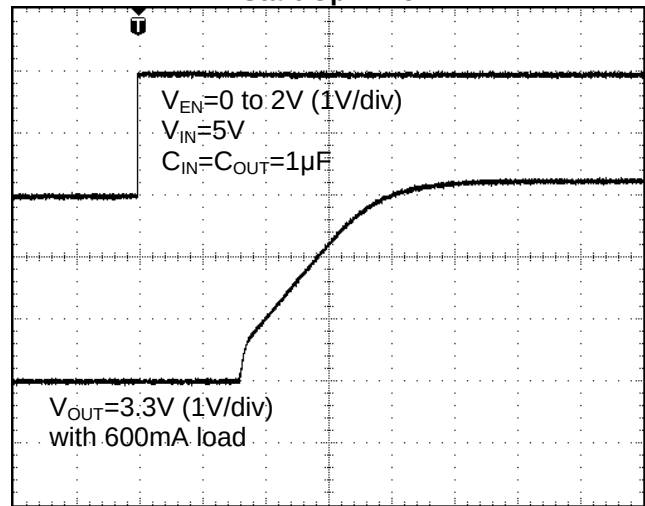
Start-Up Time
